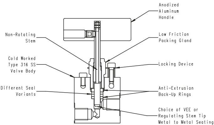
Valve Shown: 15V4B071
